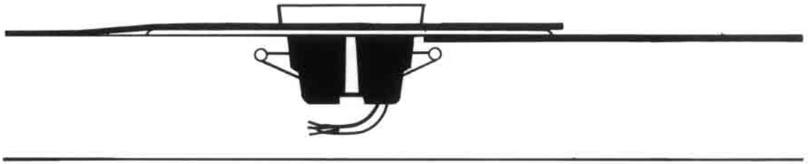
QUICKFLASH Electrical 3/0 Box Flashing Panel Part # E-3/0 B
